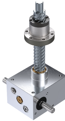
Bauart R, rotierende Spindel Type R, rotating screw
