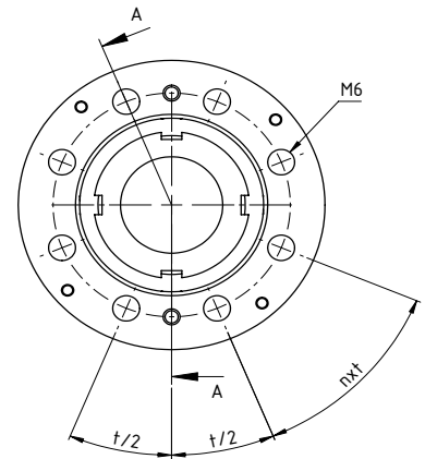
Bsp. Bohrbild ZARF40115 - nxt (12x30°) Example: Drilling pattern ZARF40115 -nxt (12x30°)
