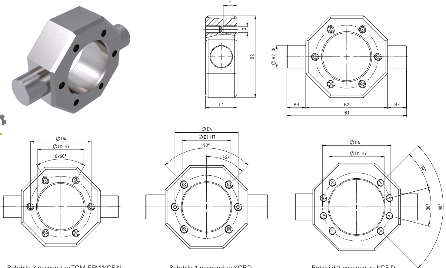
Bohrbild 3 passend zu TGM-EFM/KGF-N Drilling pattern 3 suitable for TGM-EFM/KGF-N
